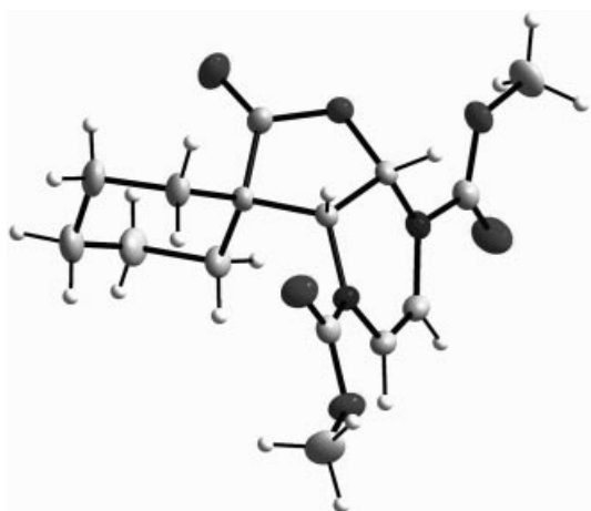
Figure 8. DIAMOND view of compound 96c .
