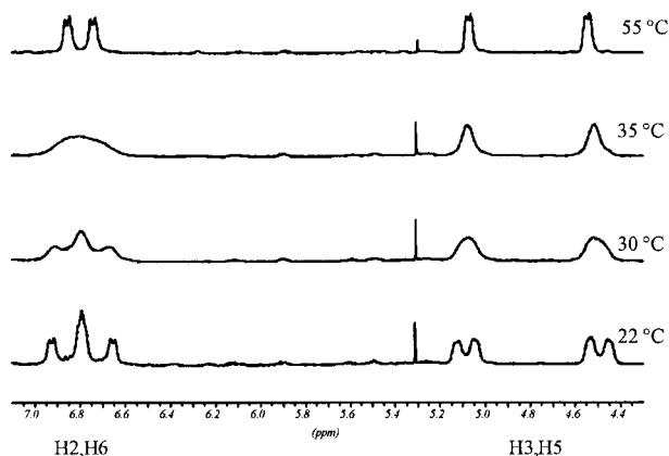
Figure 1. 1 H NMR (400 MHz) spectra of 12h at various temperatures.
